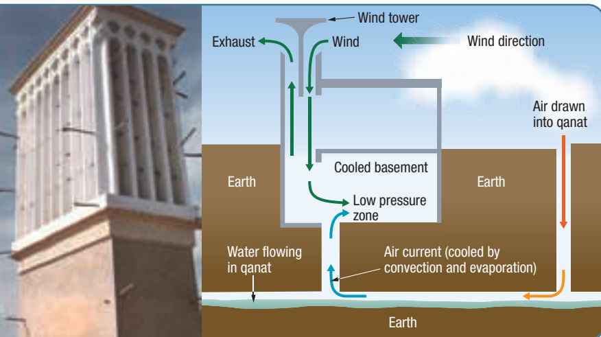
Wind catcher systems, with new technology
